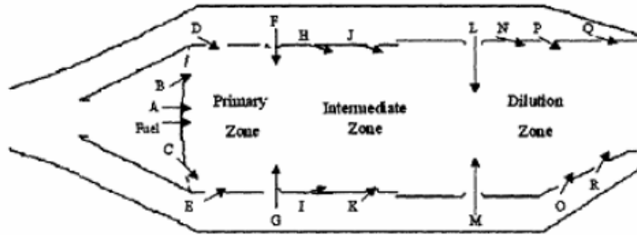
Figure 2-9: Typical Combustor Flow Splits
