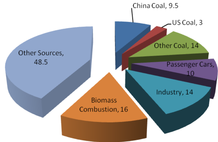
World Anthropogenic NOx Emissions, 2010 (Million Tons/Yr)
