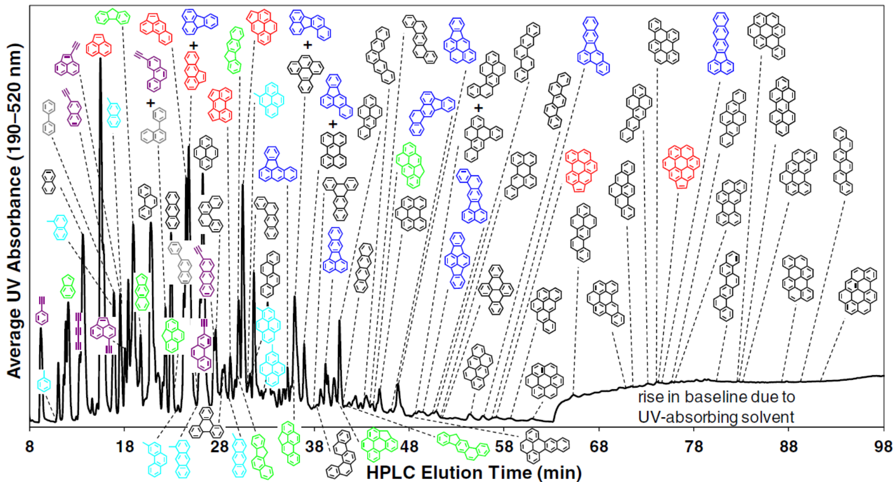
□ HPLC chromatogram of the PAH products of 1,3-butadiene/propyne co-pyrolysis
