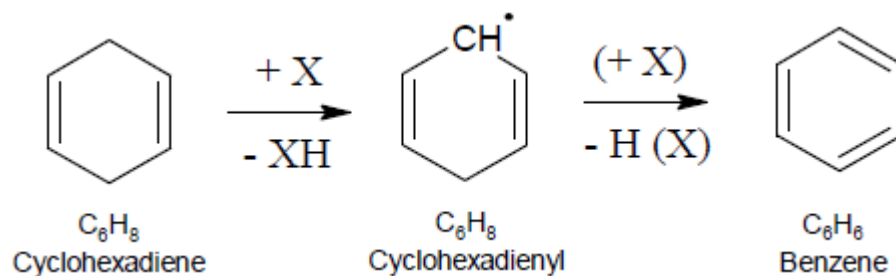
(a) Fuel-Rich Flame
