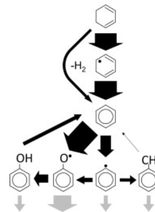
(b) Stoichiometric Flame
